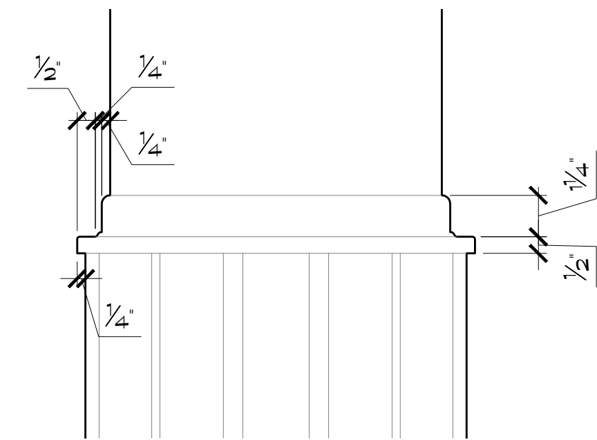
Typical Column Detail Scale: 3" = 1'-0"
