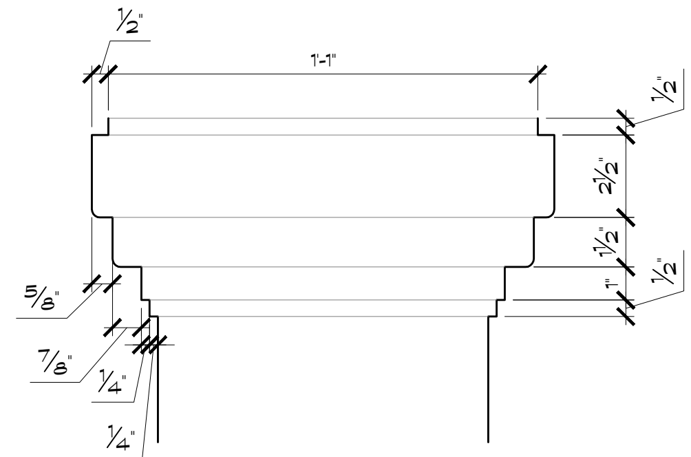
Typical Column Detail Scale: 3" = 1'-0"
