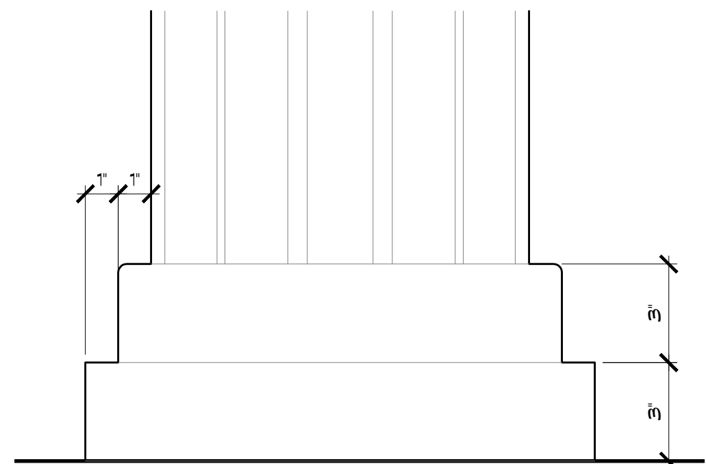
Typical Column Detail Scale: 3" = 1'-0"
